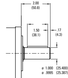
NemaTRUE PLUS* (NTP) HeavyDuty Output Shaft
